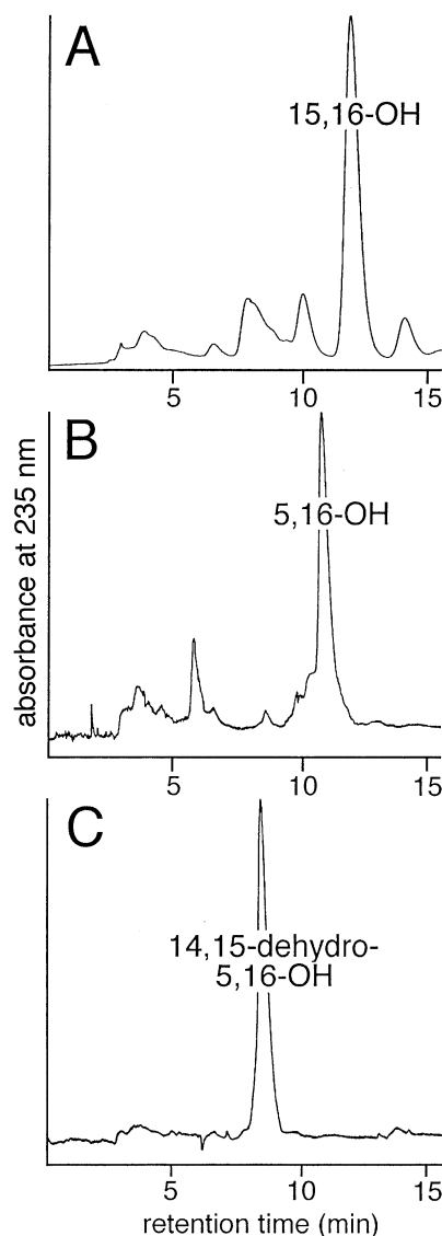
Figure 3. RP-HPLC analysis of the oxygenation products. The free acids of the lipoxygenase products were methylated with diazomethane and analyzed by RP-HPLC with a solvent system MeOH/H 2 O/acetic acid (75:25:0.1, by vol) and a flow rate of 1 mL/min: (a) 16-HETE (15) oxygenation by the soybean LOX; (b) 16-HETE (15) oxygenation by the recombinant human 5-LOX; (c) oxygenation of methyl ester of 14,15-dehydro-16-HETE (14) by the soybean lipoxygenase-1.
