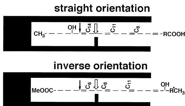
Scheme 2. Two principal possibilities for substrate orientation at the active site of lipoxygenases. For straight orientation the substrate slips into the substrate binding pocket with its methyl end ahead (upper panel). In contrast, the carboxylate slides in first for inverse head to tail substrate alignment (lower panel). The black squares indicate the catalytic non-heme iron that is responsible for hydrogen abstraction. Thick open arrows: site of initial hydrogen abstraction; thin solid arrows: site of oxygen insertion.
