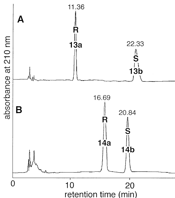
Figure 2. Enantiomer separation of (a) methyl rac-(5Z,8Z,11Z,14Z)-16-hydroxyeicosa-5,8,11,14-tetraenoate ( 13 ), and (b) methyl rac-(5Z,8Z,11Z)-16-hydroxyeicosa-5,8,11-trien-14-ynoate ( 14 ). For the analysis, a Chiralpack AD column (250×4.6 mm) from Daicel Chemical Industries was used. Solvent system: n -hexane/MeOH (98:2; by vol), flow rate 1 mL/min.
