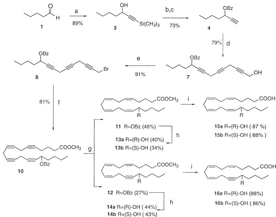
Scheme 1. (a) TMSCH≡CH ( 2 ), n -BuLi, THF, −78 °C, 0.5 h; (b) BzCl, Py, benzene, rt, 10 h; (c) n -Bu 4 NF, THF, rt, 2 h; (d) 6 , CuI, NaI, K 2 CO 3 , DMF, rt, 12 h; (e) CBr 4 , PPh 3 , CH 2 Cl 2 , rt, 1 h; (f) 9 , CuI, NaI, K 2 CO 3 , DMF, rt; (g) H 2 /Lindlar's catalyst, quinoline, benzene, 10 °C then reverse-phase HPLC; (h) MeOH, rt then chiral phase HPLC; (i) LiOH, MeOH–H 2 O, rt.
