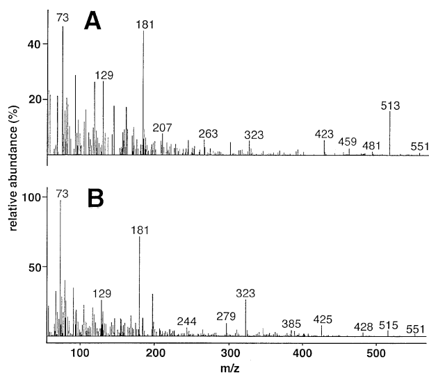
Figure 1. Mass spectra (electron ionization, 70 eV) of the pentafluorobenzyl-TMS-derivatives of rac-(5Z,8Z,11Z)-16-hydroxyeicosa-5,8,11-trien-14-ynoic acid ( 16 ) and rac-(5Z,8Z,11Z,14Z)-16-hydroxyeicosa-5,8,11,14-tetraenoic acid ( 15 ) (B). The analysis was performed as described in the Experimental.
